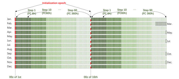
Fig. 1. Graphical representation of 15-day forecast using 2022 data. Each small square represents an epoch; the red square represents the initial epoch, which is obtained from ERA5; and the green square represents the forecast epoch, which is obtained from the forecast.
