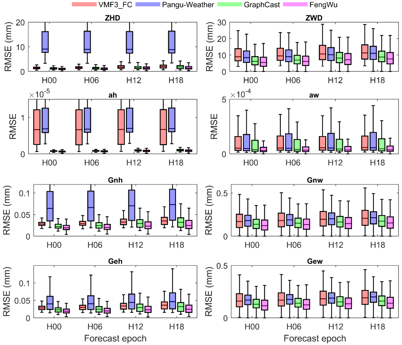
Fig. 4. RMSE of global zenith delays (ZHD and ZWD), mapping functions (ah and aw), and gradients (Gnh, Gn, Geh, and Gew) derived from VMF3_FC, Pangu-Weather, GraphCast, and FengWu FMs. Note that due to the spatial inhomogeneity of the grid, the above RMSE is latitude-weighted, and the different forecast epoch corresponds to different forecast lengths, as shown in Table III.
