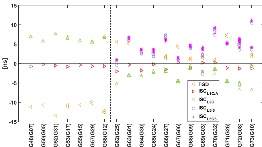
Figure 3. GPS broadcast TGD and ISC values of each individual satellite (January 2016 – March 2018). The vertical line separates Block IIR-M satellites (G48-G58) from Block IIF satellites (G62-G73). Multiple values exist for some parameters of the same satellites, which demonstrate small parameter variations during each updating.
