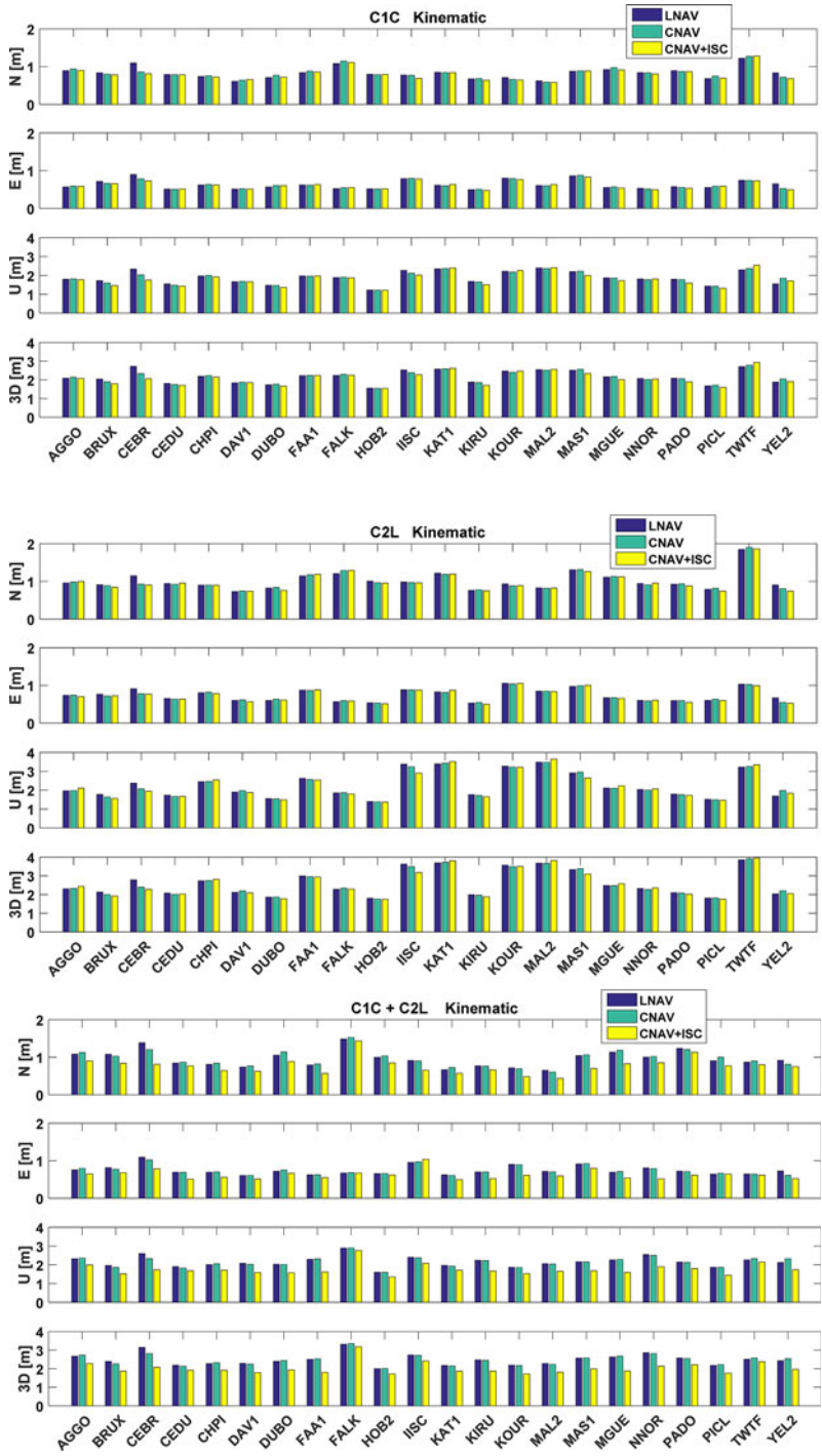
Figure 7. RMS of positioning errors in north-south, east-west, up and 3D components for 22 MGEX stations in different SPP schemes.
