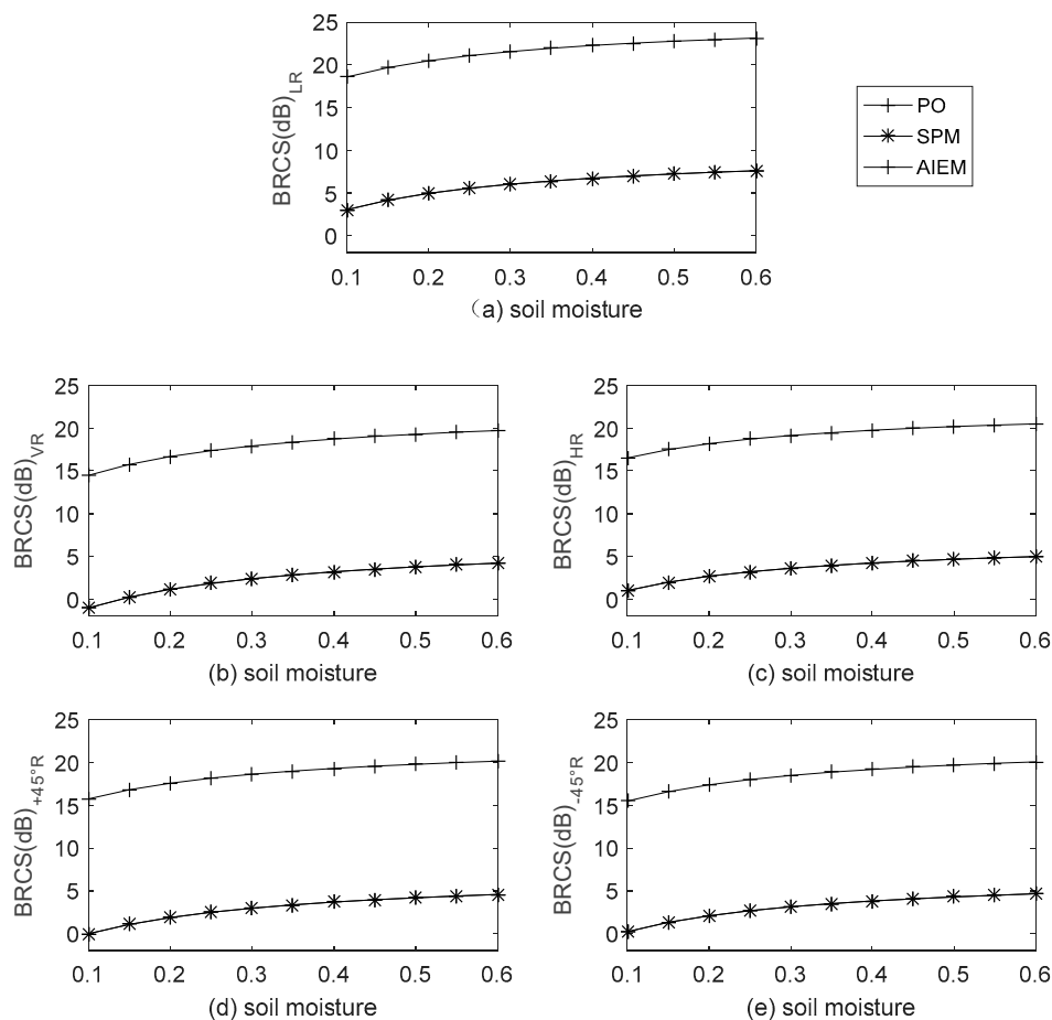
Figure 4. Soil moisture effects on BRCS at five different polarizations. \theta_i = 30, \theta_s = 30, \varphi_s = 0 . Subfigures a to e represent the polarizations of LR, VR, HR, +45° R and -45° R, respectively.
