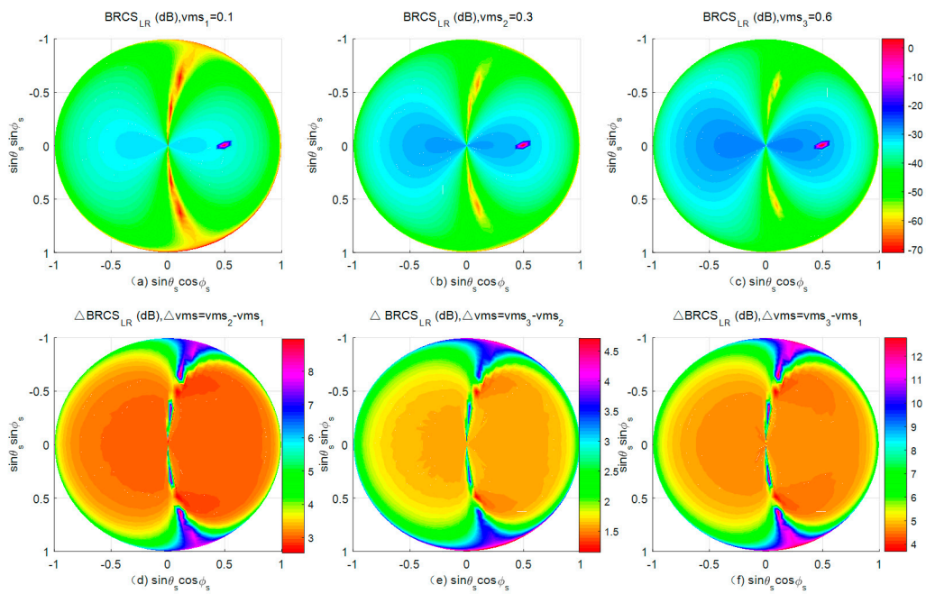
Figure 8. BRCS for different soil moisture contents (a–c) and the BRCS differences for different soil moisture differences (d–f) at LR polarization.
