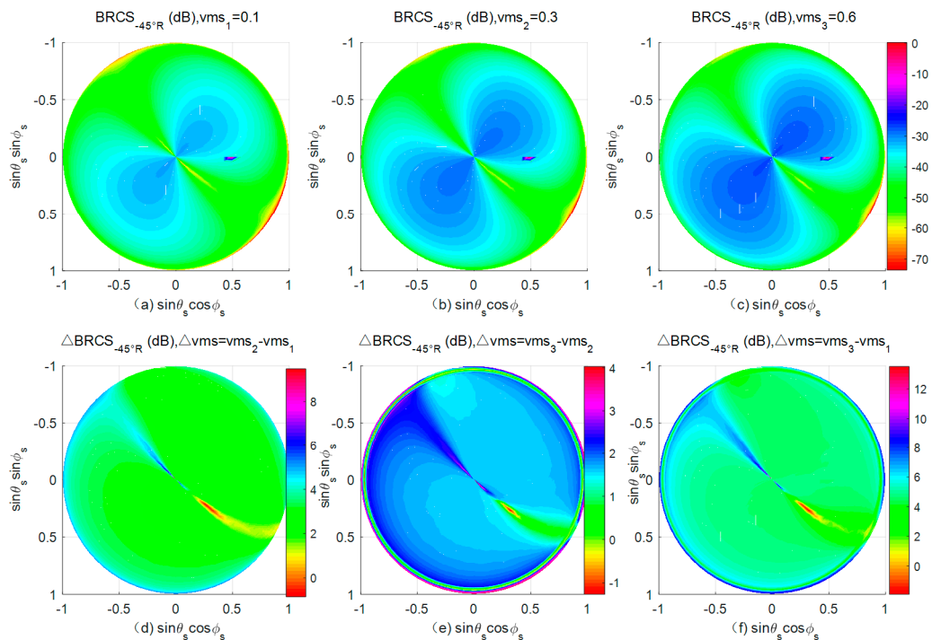
Figure 12. BRCS for different soil moisture contents (a–c) and the BRCS differences for different soil moisture differences (d–f) at -45^\circ R polarization.
