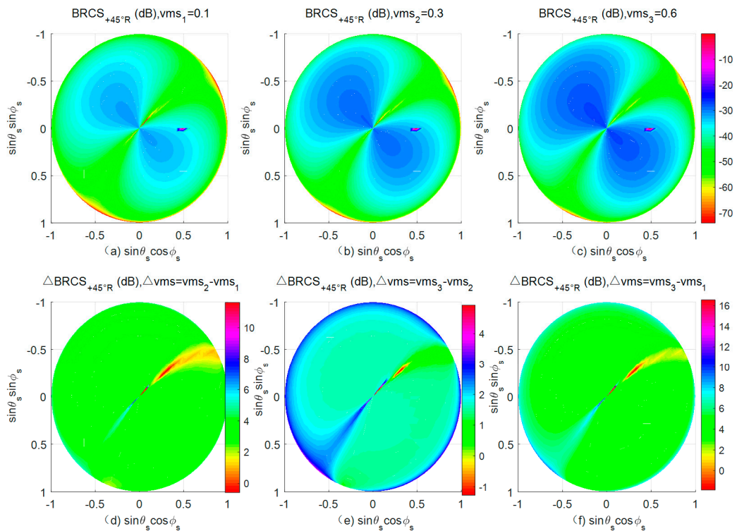
Figure 11. BRCS for different soil moisture contents (a–c) and the BRCS differences for different soil moisture differences (d–f) at +45° R polarization.
