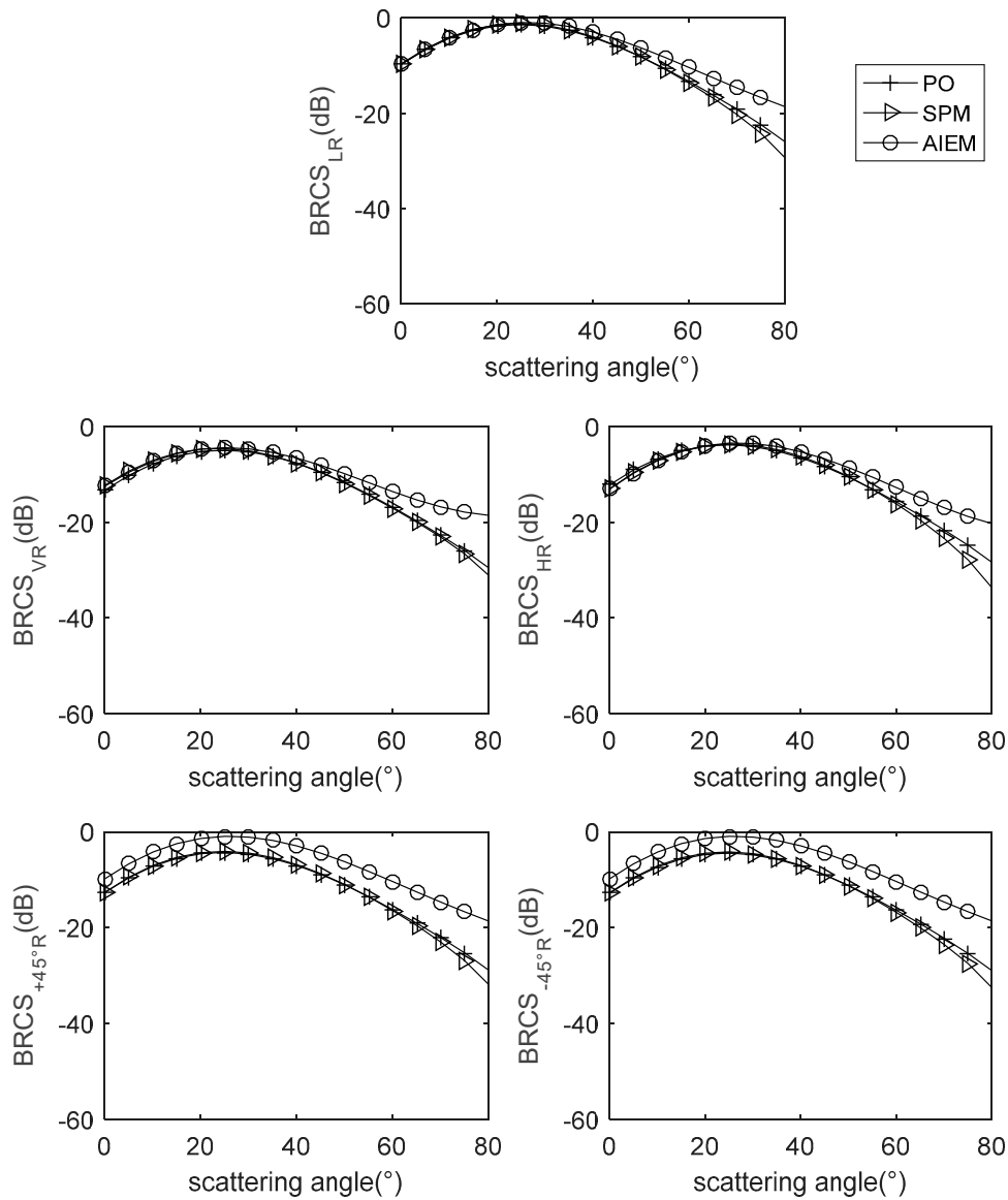
Figure 6. Scattering zenith angles’ effects on BRCS at five different polarizations. \theta_i = 30^{\circ} , \varphi_s = 0^{\circ} . Subfigures a to e represent the polarizations of LR, VR, HR, +45^{\circ} R and -45^{\circ} R, respectively.
