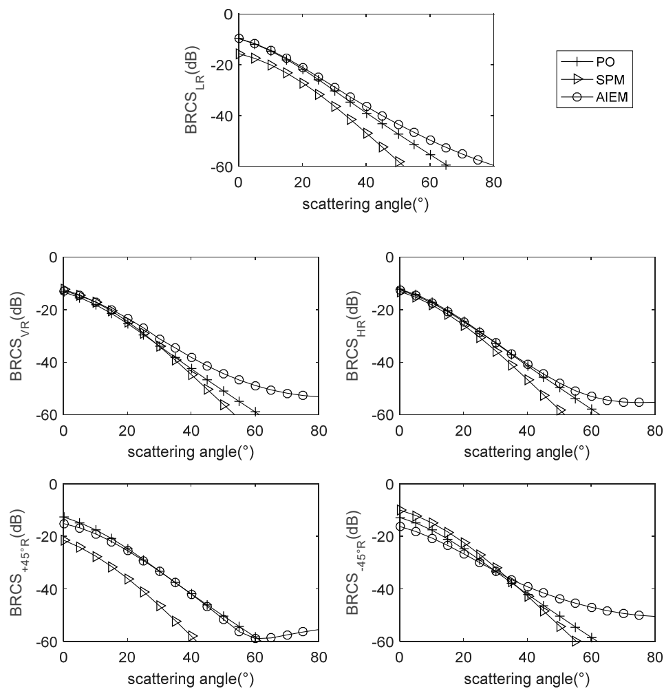
Figure 5. Scattering zenith angles' effects on BRCS at five different polarizations. \theta_i = 30^\circ , \theta_s = 30^\circ , \varphi_s = 0^\circ . Subfigures a to e represent the polarizations of LR, VR, HR, +45^\circ R and -45^\circ R, respectively.
