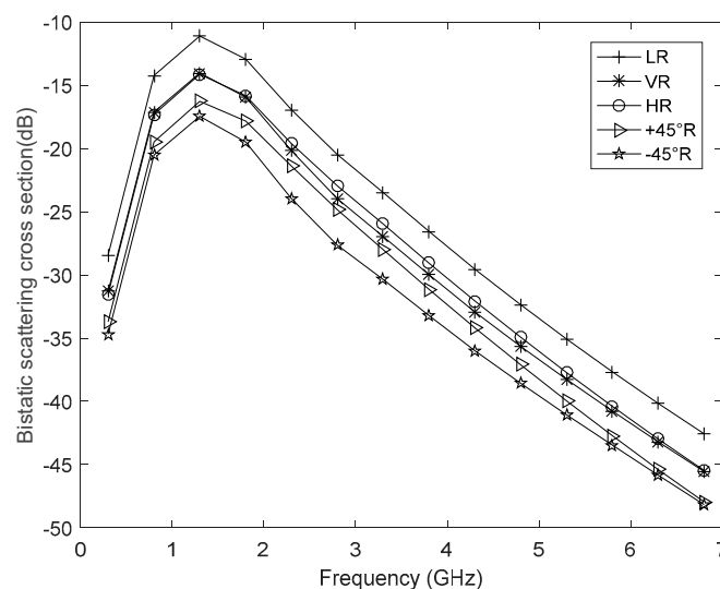
Figure 2. Variation of bistatic radar scattering cross section (BRCS) with frequency for five different polarizations.
