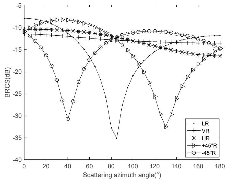
Figure 7. Scattering azimuth angles' effects on BRCS at five different polarizations.
