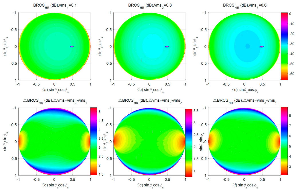
Figure 10. BRCS for different soil moisture contents (a–c) and the BRCS differences for different soil moisture differences (d–f) at HR polarization.
