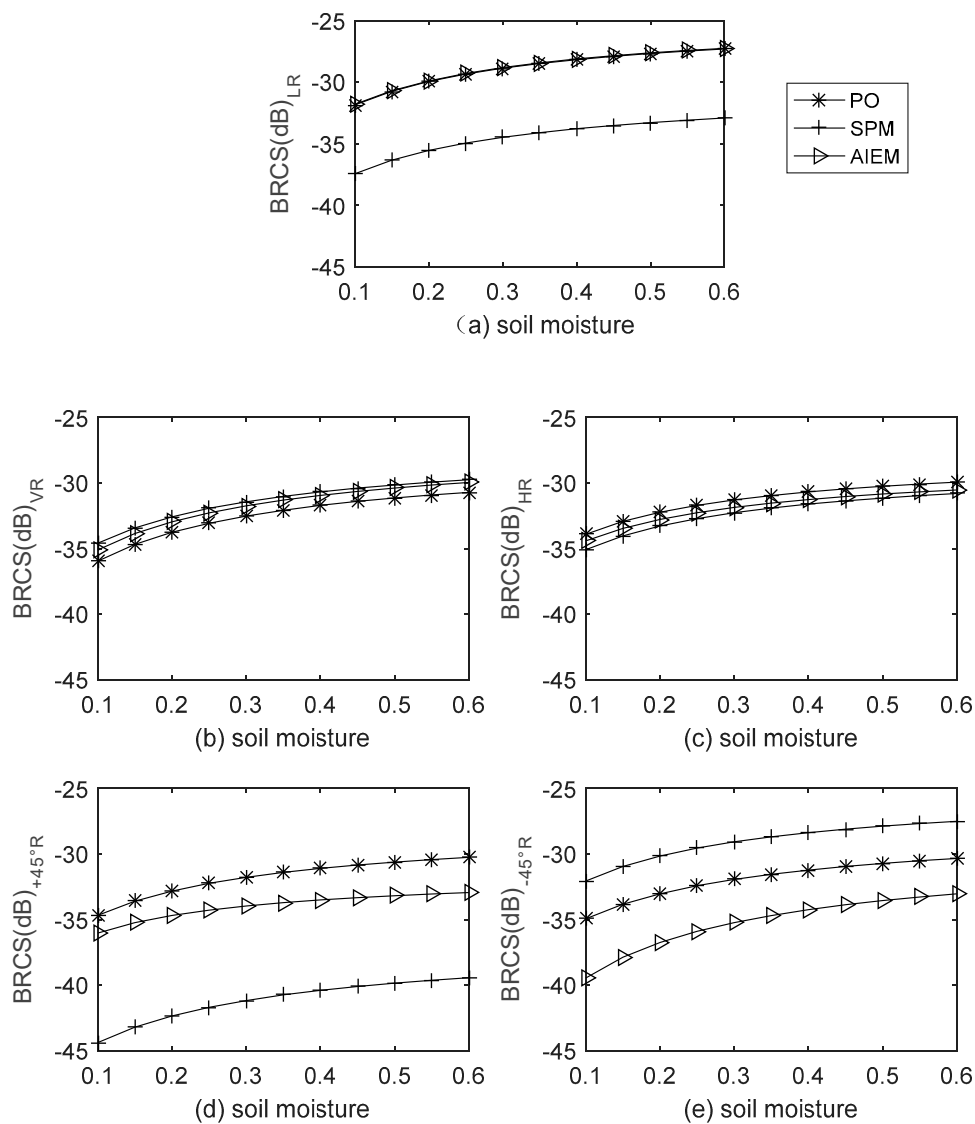
Figure 3. Soil moisture effects on BRCS at five different polarizations. \theta_i = 30, \theta_s = 5, \varphi_s = 120 . Subfigures a to e represent the polarizations of LR, VR, HR, +45^\circ R and -45^\circ R, respectively.
