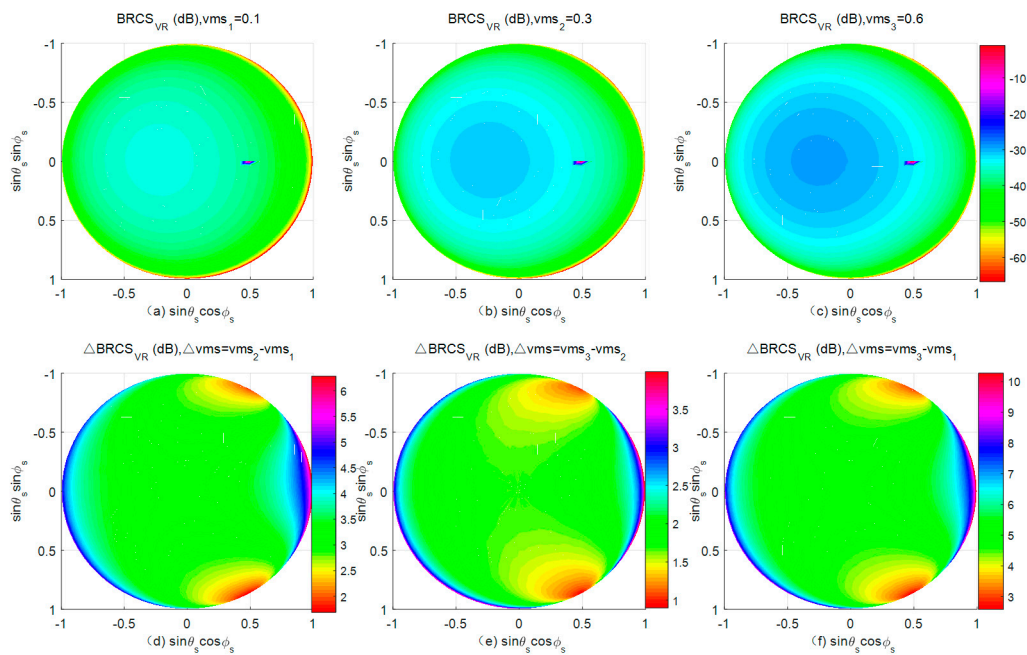
Figure 9. BRCS for different soil moisture contents (a–c) and the BRCS differences for different soil moisture differences (d–f) at VR polarization.
