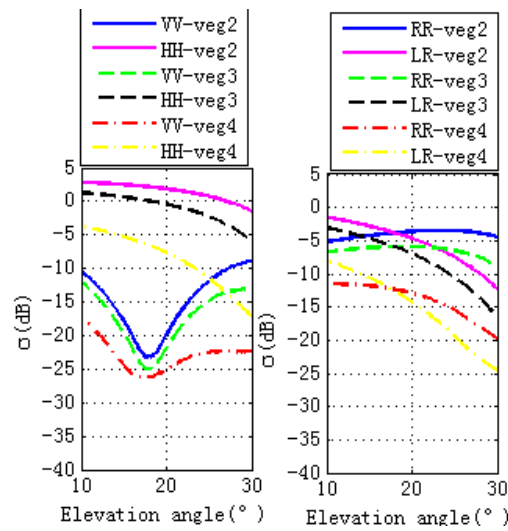
Figure 8. Specular scattering cross sections of different vegetation sizes. The left hand figure is for linear polarizations, while the right hand figure is for circular polarizations. Lengths and diameters of the stems or thicknesses and diameters of the leaves for veg 2, veg 3 and veg 4 are different. The sizes of veg 2 are smaller than veg 3, while the sizes of veg 4 are the largest.
