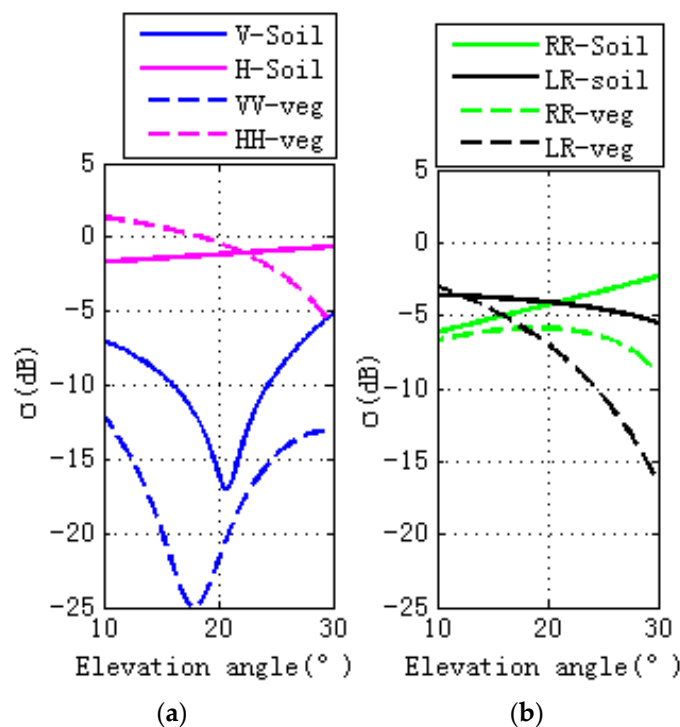
Figure 4. Specular scattering comparisons of vegetation and bare soil, (a) is for linear polarizations, while (b) is for circular polarizations. Bare soil and vegetation are shown, respectively, in solid and dashed line styles. VV pol is shown in blue, HH pol in pink
