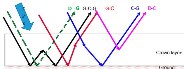
Figure 2. Scattering mechanisms in the Bi-Mimics model (only the crown layer and the ground layer are retained, while the trunk layer has been eliminated) including D-G (direct ground), G-C-G (ground reflection and crown scattering and ground reflection), G-C (ground reflection and crown scattering), C-G (crown scattering and ground reflection) and D-C (direct crown scattering). The specular ground reflection is not shown in the figure (S-G). For the same scattering mechanism, it has the same color for the arrows and the top legend.
