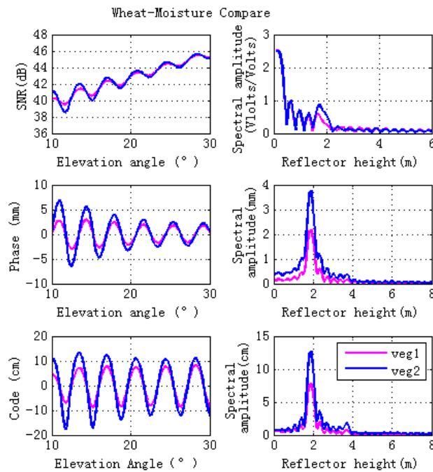
Figure 5. Effects of different vegetation moisture content on the forward GPS multipath simulation. The vegetation moisture content of Veg 1 (Vegetation 1) is higher than that one of Veg 2 (Vegetation 2). The moisture content (gravimetric) of stem and leaf for Veg 1 is 0.72 and 0.8, respectively, while the equipment for Veg 2 is 0.2 and 0.2, respectively. Veg 1 is shown in pink, Veg 2 in blue. Lomb-Sargle periodograms computed for the GPS multipath signatures are shown in the right hand panel.
