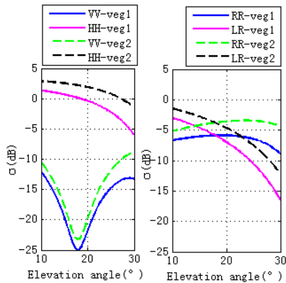
Figure 6. Specular scattering cross sections of different vegetation moisture contents. The left figure is for linear polarizations, while the right one is for circular polarizations. The vegetation moisture contents of Veg 1 (Vegetation 1) is larger than the one of Veg 2 (Vegetation 2). The moisture contents (gravimetric) of stem and leaf for Veg 1 are 0.72 and 0.8, respectively. While the ones for Veg 2 are 0.2 and 0.2, respectively.
