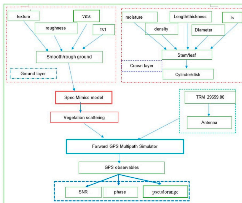
Figure 1. Flowchart of the improved forward GPS multipath simulator. The forward GPS multipath simulator (in the green box) is mainly composed of the effects of vegetation scattering and antenna type. The main improvement of the simulator is to use the Spec-Mimics model (in the red box) to represent the vegetation scattering. TRM 29659.00 is a representative of the antenna type (in the green dotted lines). Those parts in the red dotted lines are the frame of the Spec-Mimics model: ground layer and crown layer. The parameters in the red dotted line boxes are the model inputs, while the ones in the blue box are outputs of the model. Soil texture is represented by the percentages of sand and clay in soil, respectively, its roughness is characterized by rms height and correlation length. Vms is the volumetric soil moisture content, ts1 is the temperature of the soil, as for the crown layer, stem or leaf are represented by the dielectric scatters of cylinders or disks, respectively. Moisture content, density, length/thickness, diameter and temperature of the scatters are the inputs for the crown layer. SNR, phase and pseudorange are the final outputs of the simulator.
