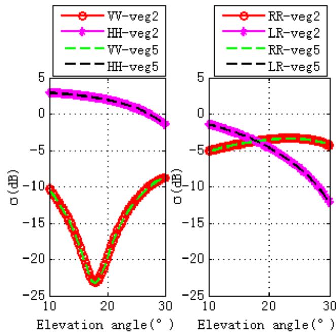
Figure 11. Specular scattering cross sections for Veg 2 and Veg 5. The ground soil moisture content for veg 2 is 0.15, while the one for veg 5 is 0.55. The left figure is for linear polarizations, while the right one is for circular polarizations.
