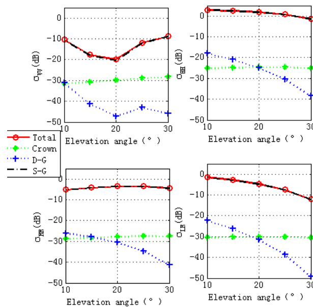
Figure 9. Vegetation scattering component contributions versus the specular incidence angles. The top panel is for linear polarization (VW and HH) and the bottom panel is for circular polarization (RR and LR). Total is the total scattering; Crown is the scattering from the crown layer; D-G is the Direct-ground scattering component; and S-G is the specular scattering component.
