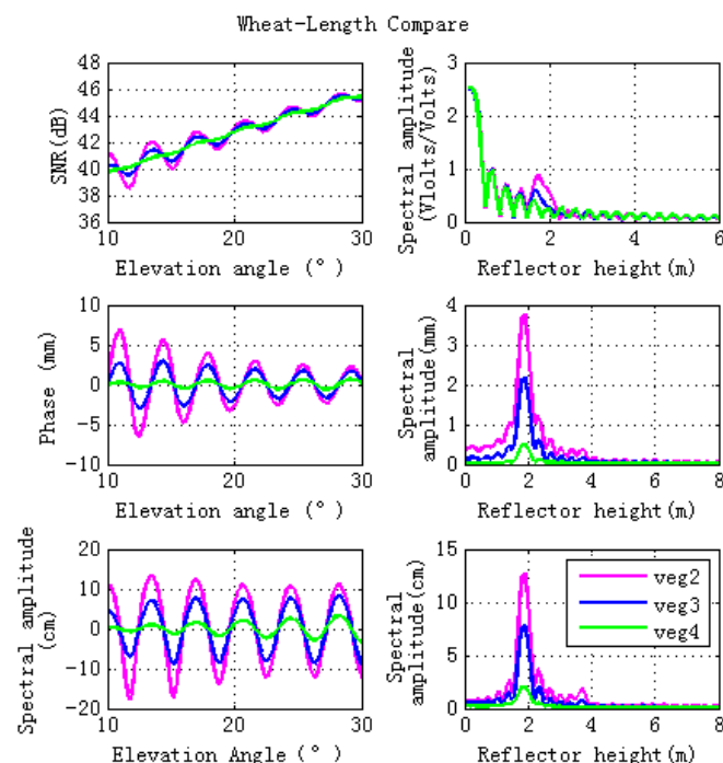
Figure 7. Effects of different vegetation sizes on the forward GPS multipath simulation observables. The lengths and diameters of the stems or the thicknesses and diameters of the leaves for Vegetation 2 (veg 2), Vegetation 3 (veg 3) and Vegetation 4 (veg 4) are different. The sizes of veg 2 are smaller than veg3, while the sizes of veg 4 are largest. Results for varying wheat lengths are shown in pink (veg 2), blue (veg 3) and green (veg 4). Lomb-Sargle periodograms computed for the GPS multipath signatures are shown in the right panel in plots.
