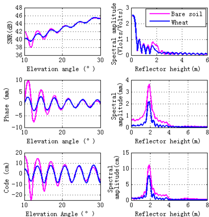
Figure 3. Comparisons of GPS multipath simulation between vegetation (veg) and bare soil (soil). Model inputs for bare soil are the same as the ground layer of vegetation. Bare soil is shown pink, wheat in blue. Lomb-Sargle periodograms computed for the GPS multipath signatures are shown in the right panel in plots.
